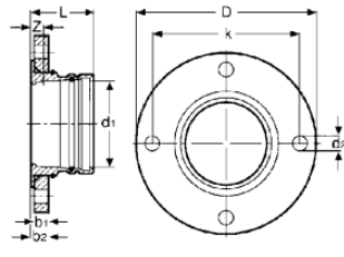
XL 2-1/2"- 4"
