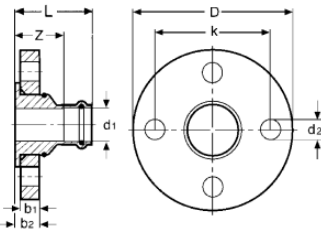
Sizes 1", 1-1/4", 1-1/2" and 2"
